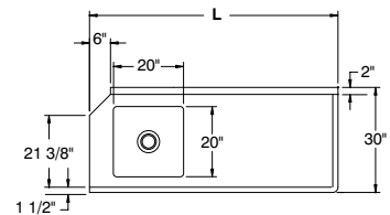
RIGHT SOIL TABLE
