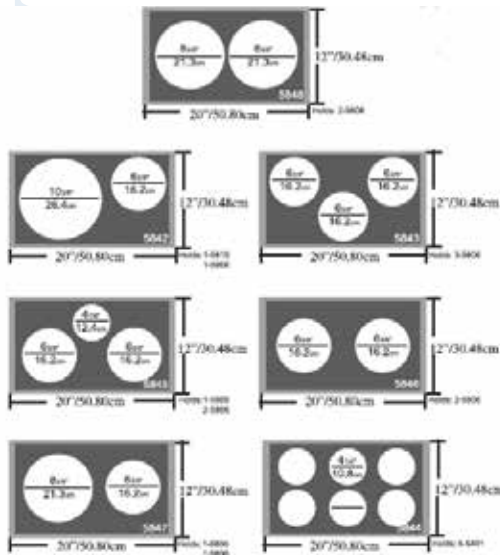
ADAPTOR PLATE CUTOUT DIMENSIONS
